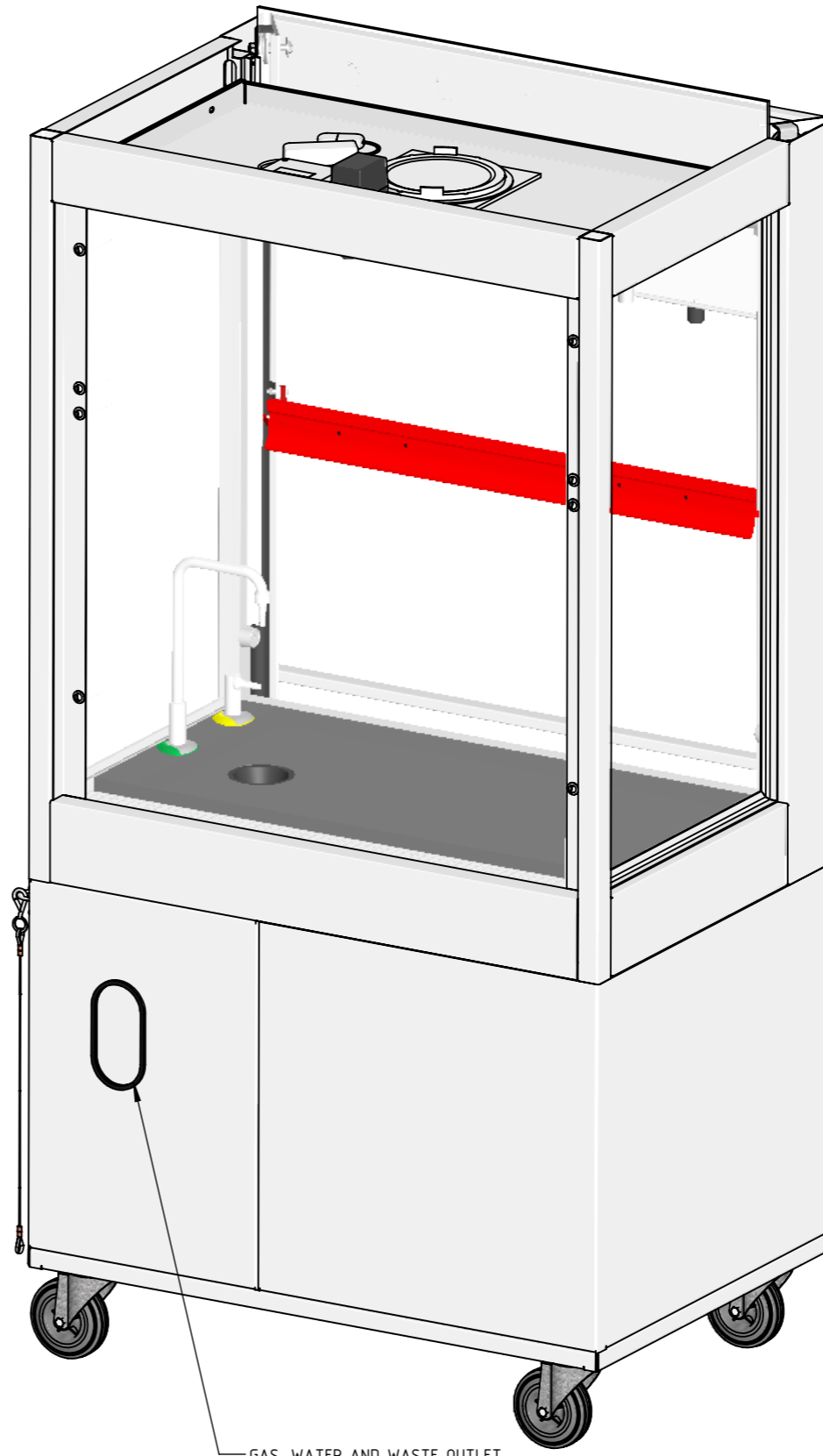
VIEW ON REAR
