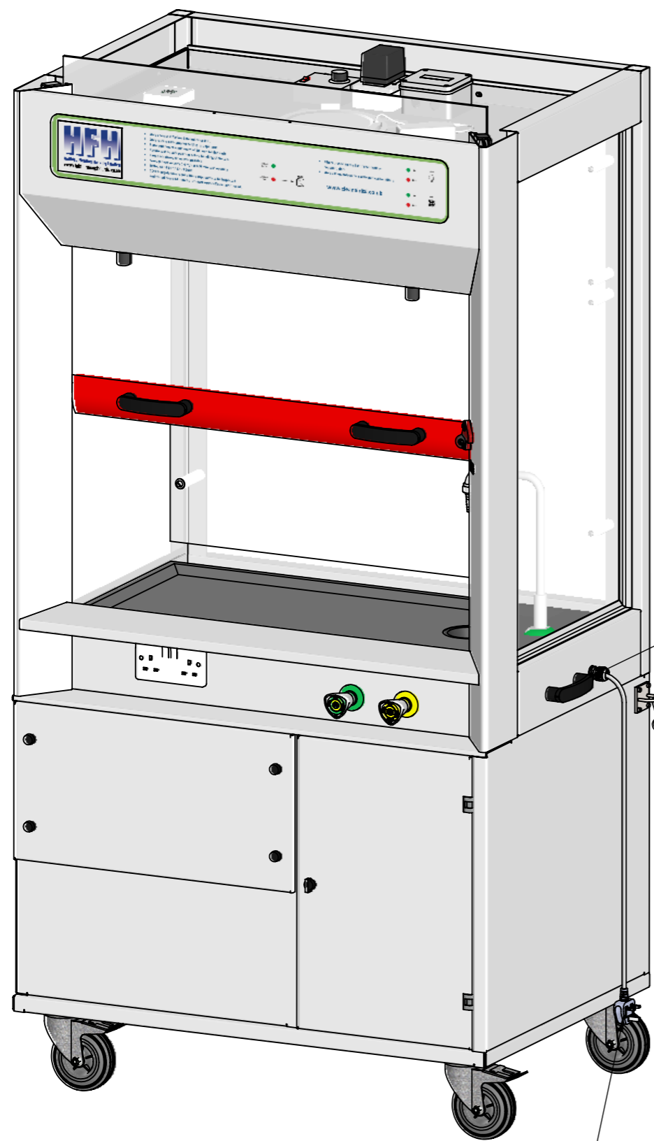
VIEW ON FRONT
