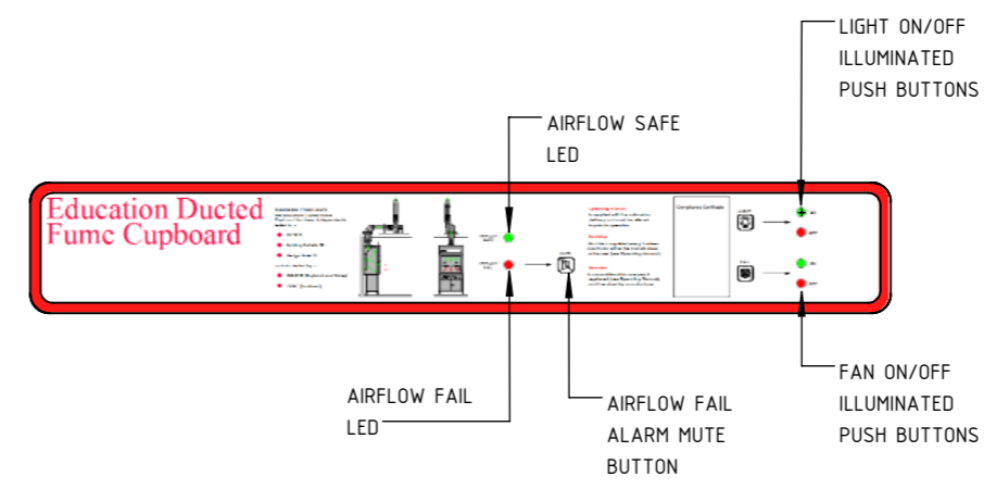
FUME CUPBOARD CONTROL PANEL FASCIA
