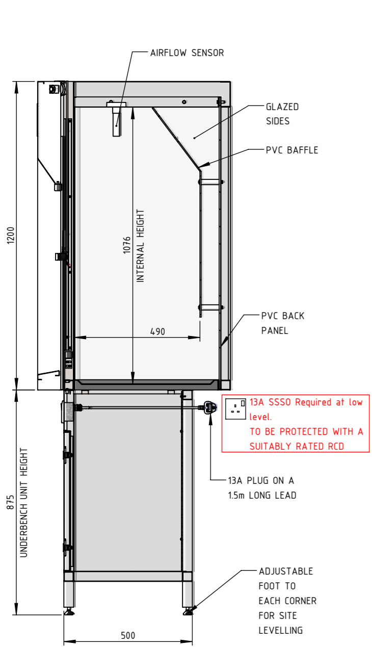
L.H. SECTIONAL ELEVATION
