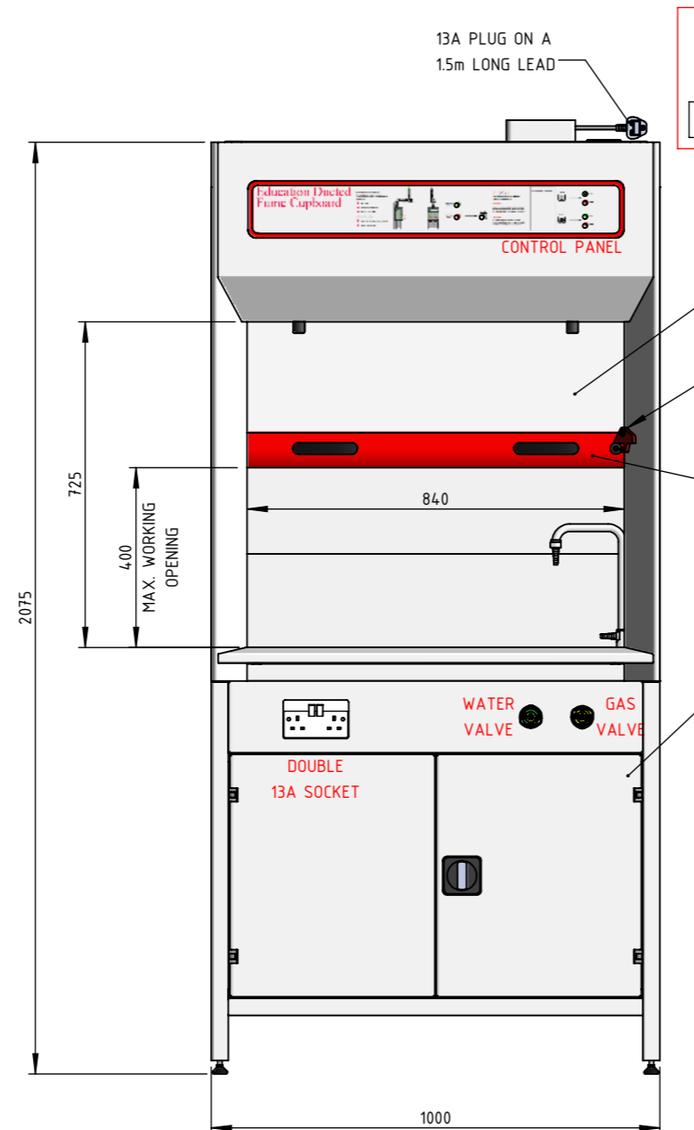
FRONT ELEVATION
