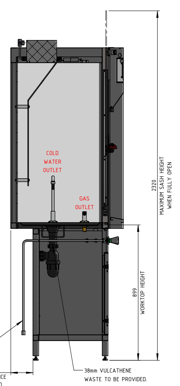
R.H. SECTIONAL ELEVATION
